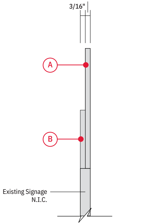
2 DN-01A Room Sign Small Section View
