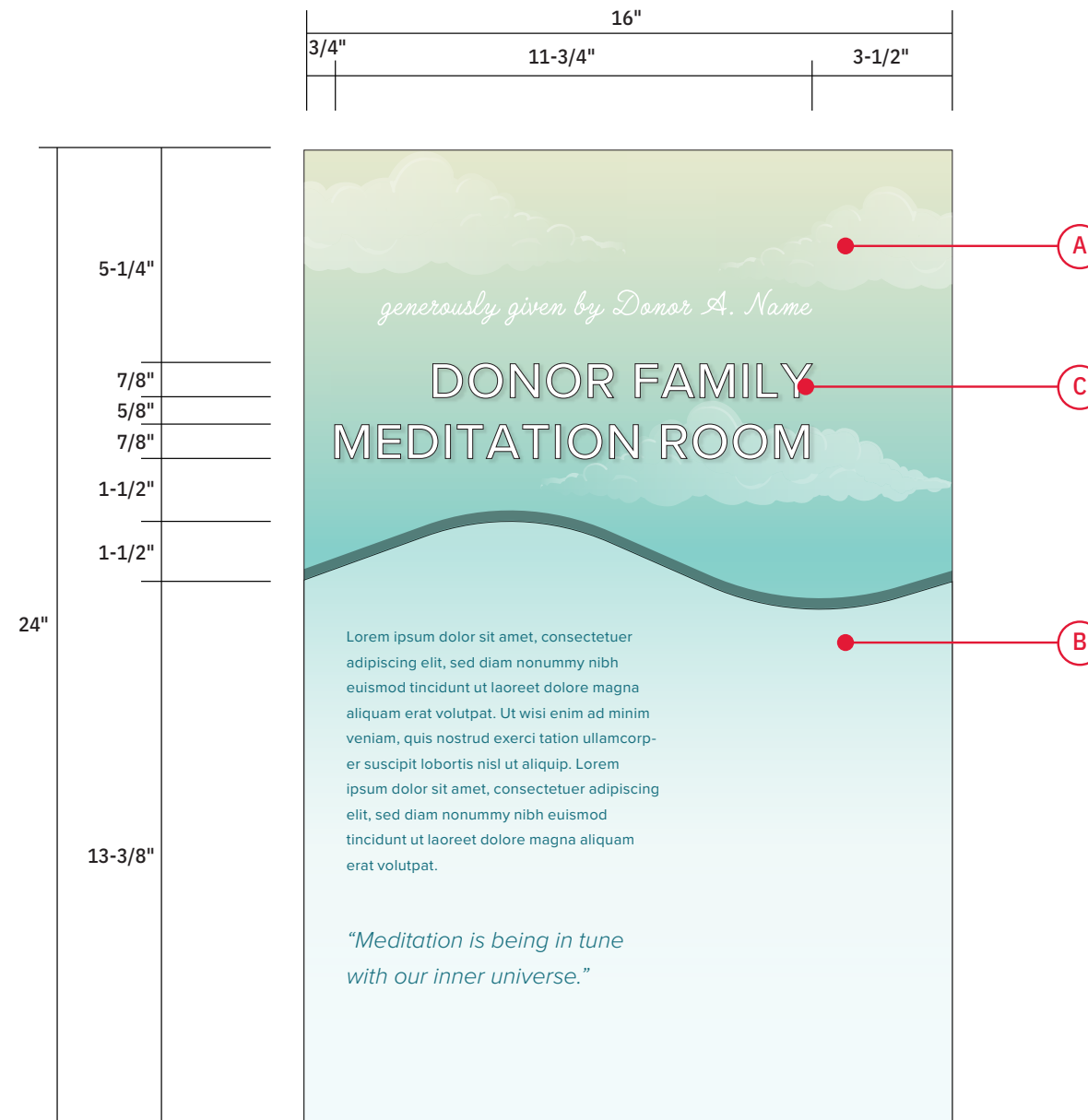
1 DN-03 Donor Story Panel Front Elevation Scale: 3" = 1'-0"
