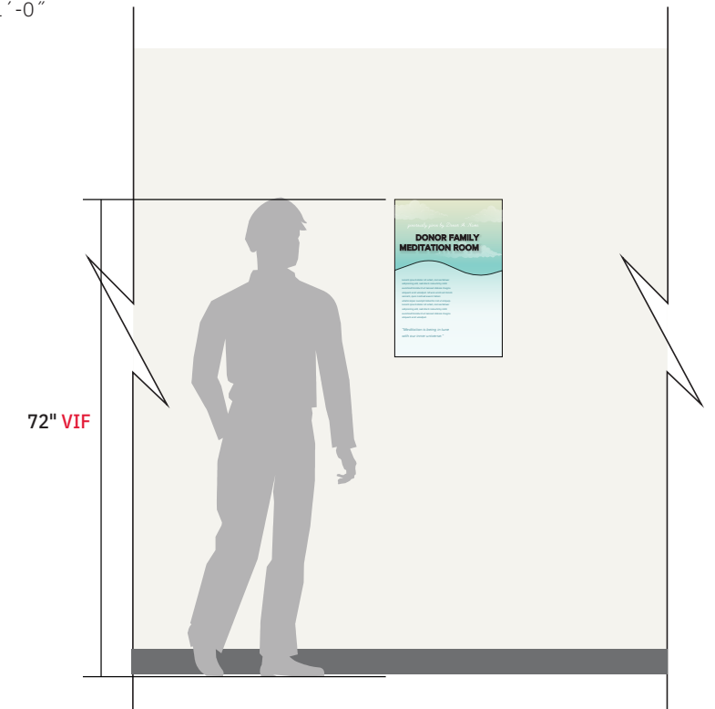
3 DN-03 Donor Story Panel Mounting Elevation Scale: 1/2" = 1'-0"
