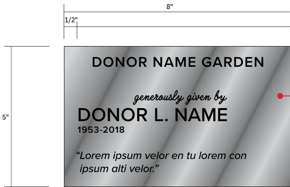
1 DN-07 Sculpture Donor Plaque Front Elevation Scale: 6" = 1'-0"
