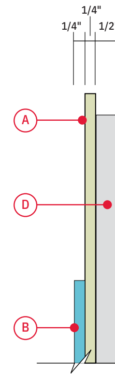
2 DN-03 Donor Story Panel Section View Scale: 6" = 1'-0"
