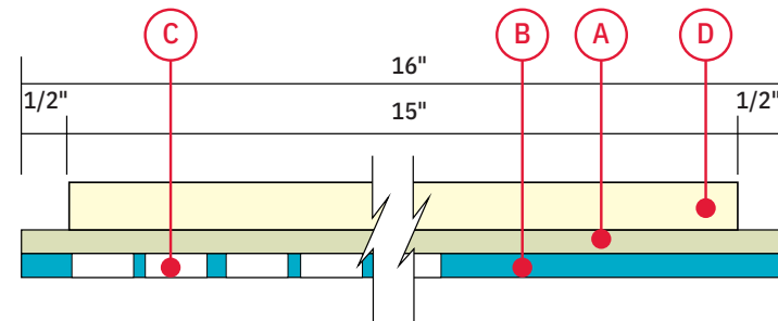
2 DN-03 Donor Story Panel Plan View Scale: 6" = 1'-0"
